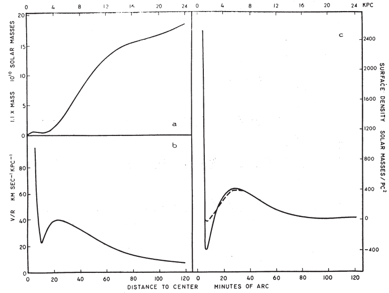
FIG. 10.—(a) Total mass of M31 out to R = 24 kpc determined from rotation curve (Fig. 9), as a function of distance from the center, and multiplied by 1.1 to compensate for flat disk approximation. (b) Angular velocity, V/R , for M31, calculated from rotation curve, as a function of distance from center. (c) Surface density for M31, determined from rotation curve, as a function of distance from center. Solid curve and dashed curve are calculated from corresponding curves in Fig. 9.
