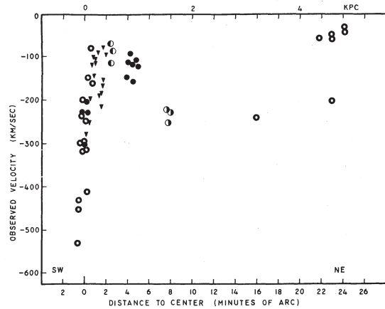
FIG. 6.—Observed velocities along the NE major axis of M31 from the [\text{N II}] \lambda 6583 emission line. For R \leq 8' , different symbols represent different plates. For R > 15' , open circles indicate velocities of innermost emission regions.
